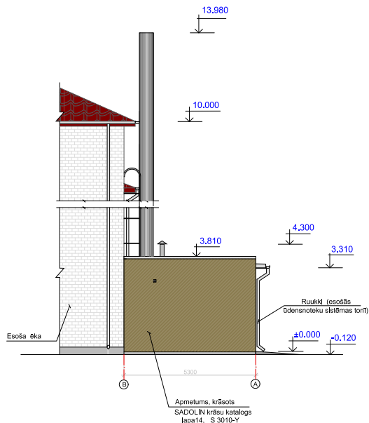
FASĀDES FRAGMENTS assis B-A. M 1:100.
