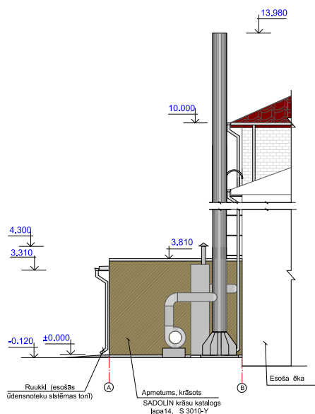
FASĀDES FRAGMENTS assis A-B. M 1:100.
