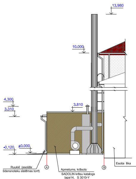
FASĀDES FRAGMENTS asis A - B. M 1:100.
