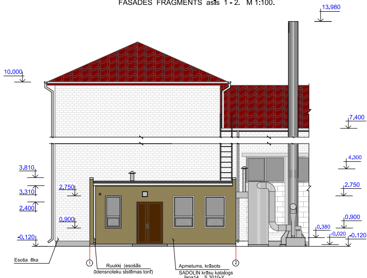
FASĀDES FRAGMENTS assis 1-2. M 1:100.
